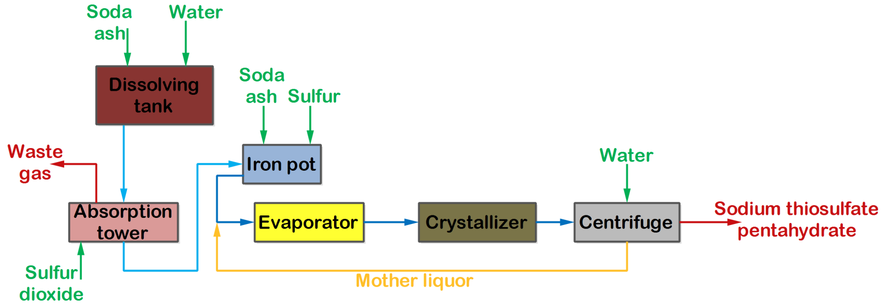
Figure: Manufacture of Sodium thiosulfate from soda ash and sulfur dioxide
